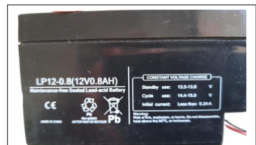
MF Sealed Lead Acid Battery LP12-0.8 (12V 0.8AH)-BAT8010 L=9.5 cms. W=2.4 cms. H=6.1 cms.
